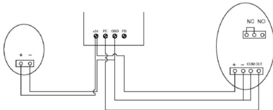
Connection of photo beam/switch control
