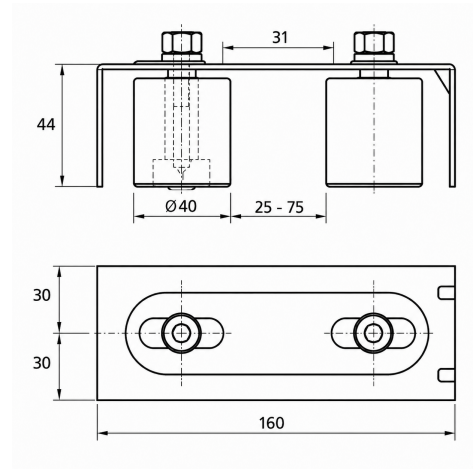
Dimensions (mm)
