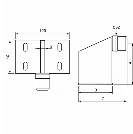
Dimensions (mm)
