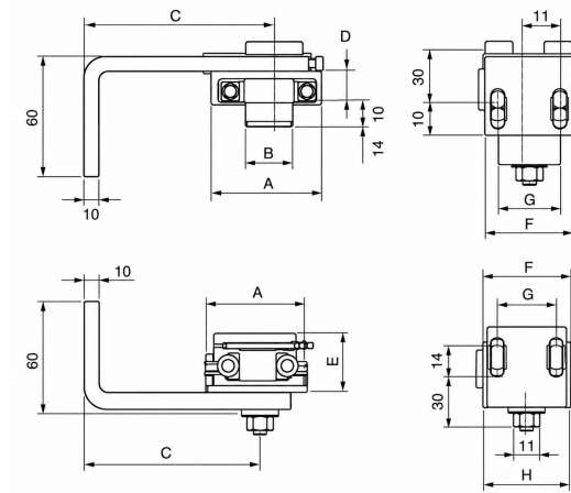
Dimensions (mm)
