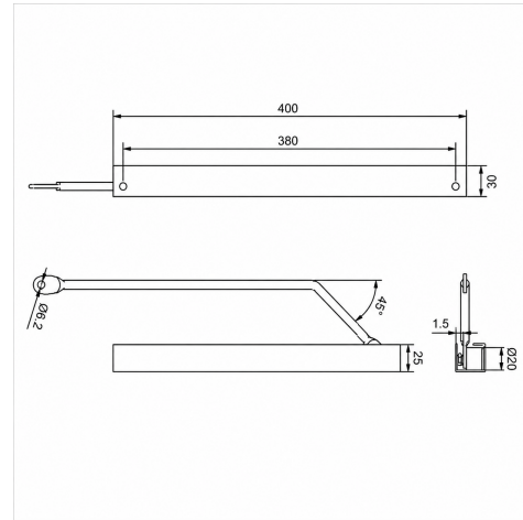
Dimensions (mm)
