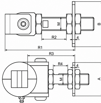
Dimensions (mm)
