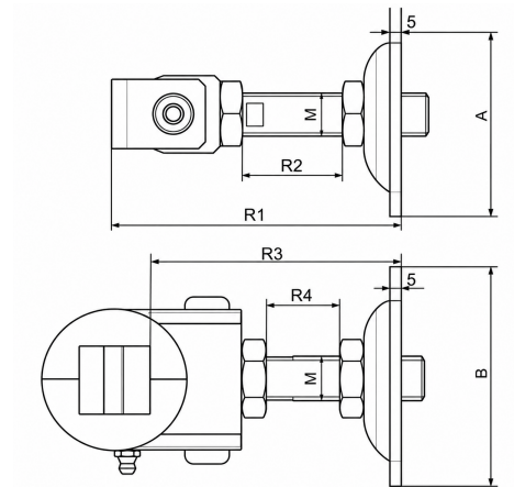
Dimensions (mm)
