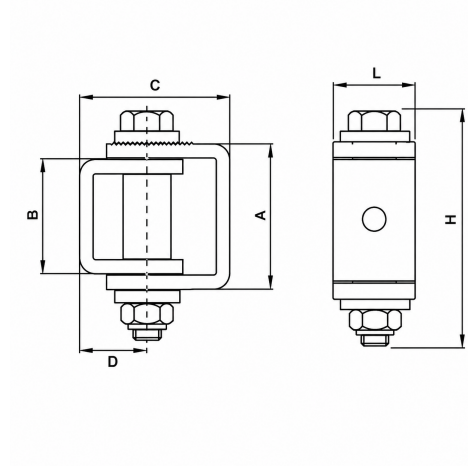
Dimensions (mm)
