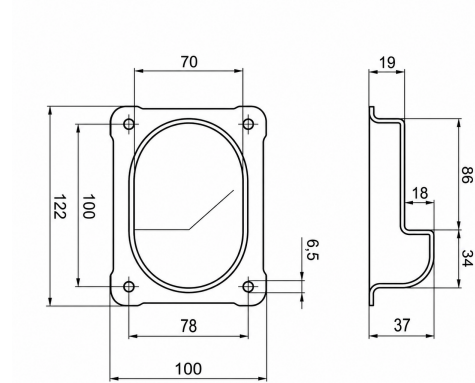
Dimensions (mm)
