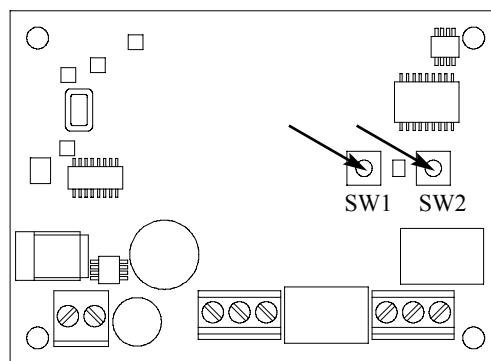
CRX-2 Stand Alone Receiver
